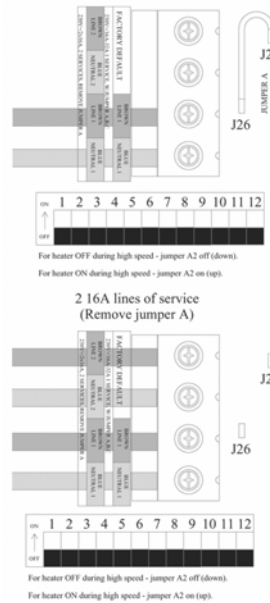
Single 32A line of service.
